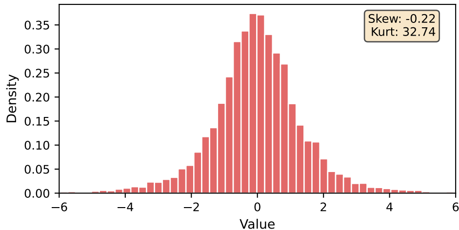
t(df=3): Heavy-Tailed
