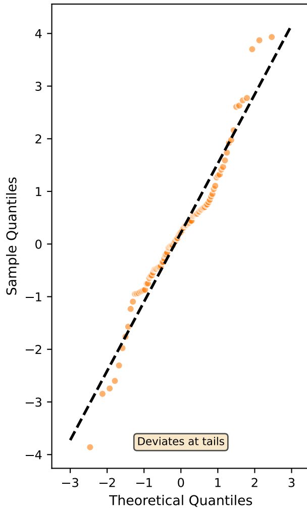
Heavy-Tailed (t, df=3)
