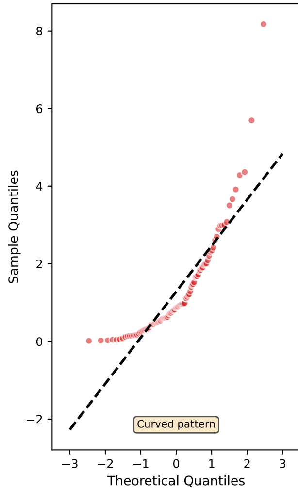
Right-Skewed (Exp)
