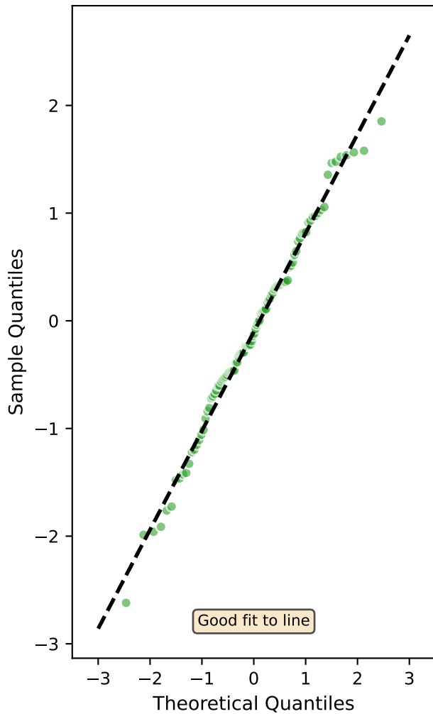
Normal Data
