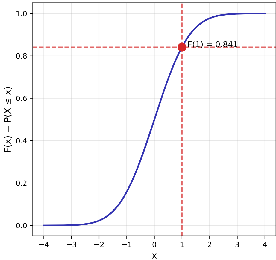
CDF: F(x)
