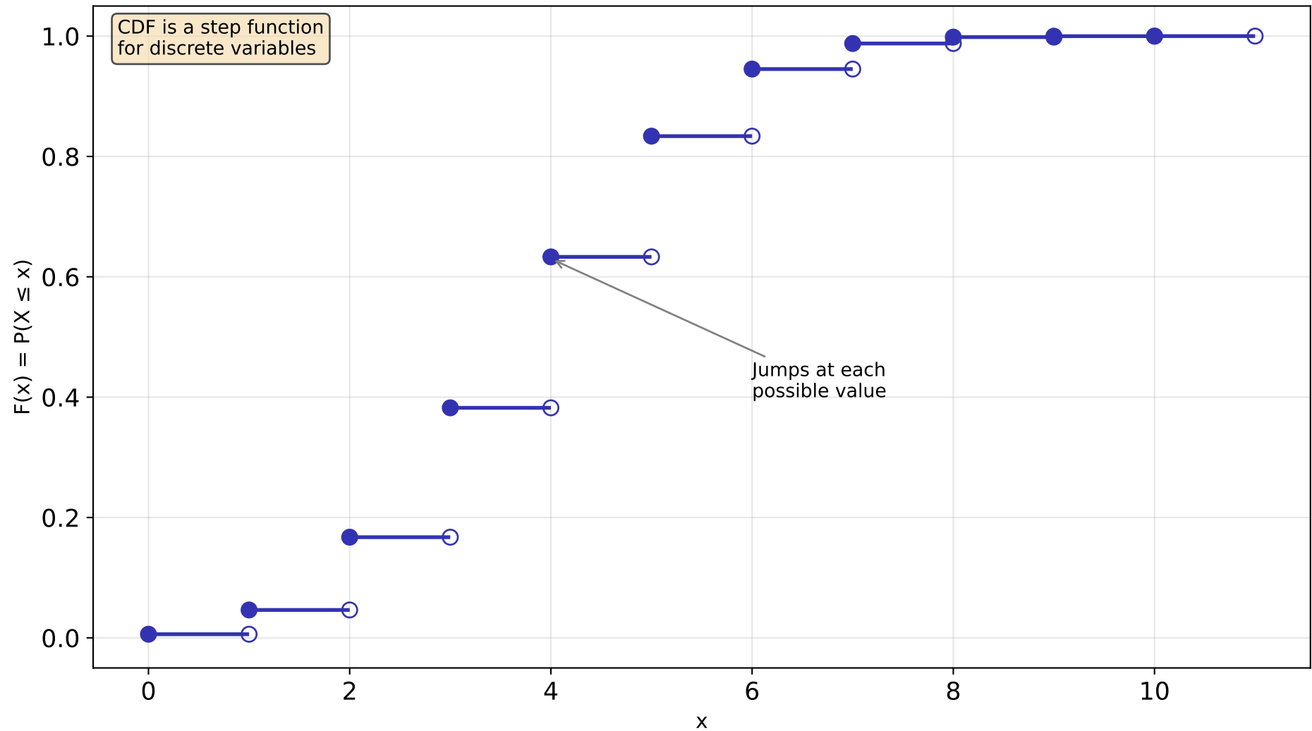
CDF of Binomial( n=10 , p=0.4 )
