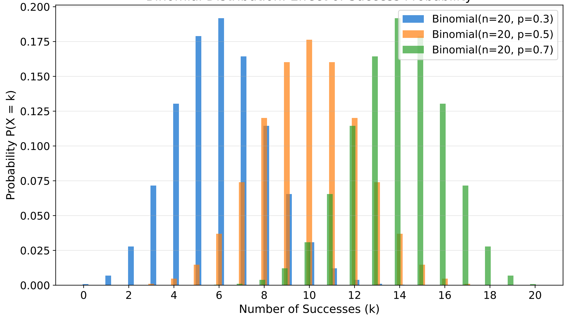
Binomial Distribution: Effect of Success Probability
