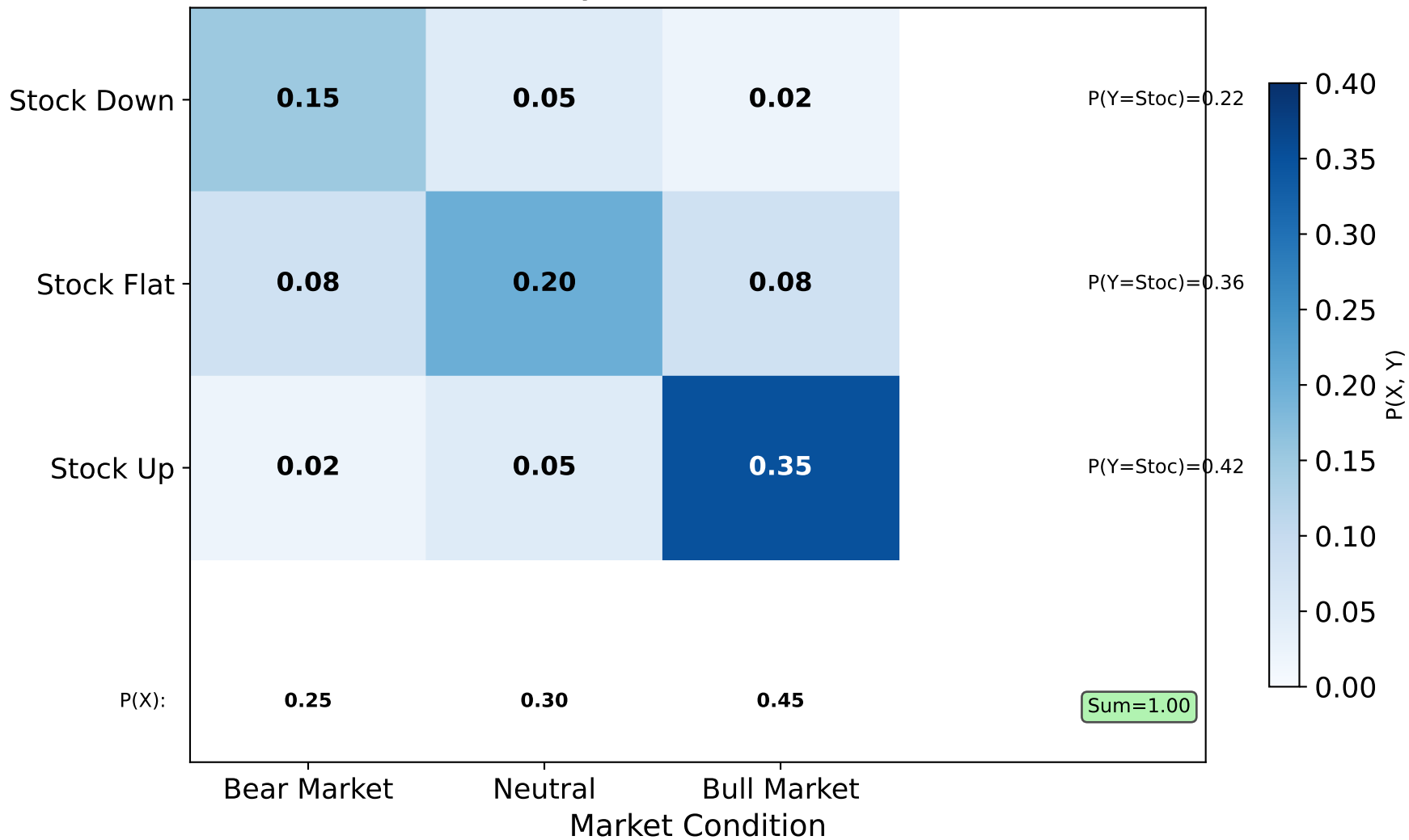
Joint Probability Distribution P(Stock, Market)
