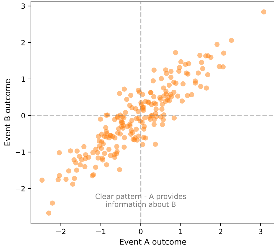
Dependent Events P(A \text{ and } B) \neq P(A) * P(B)
