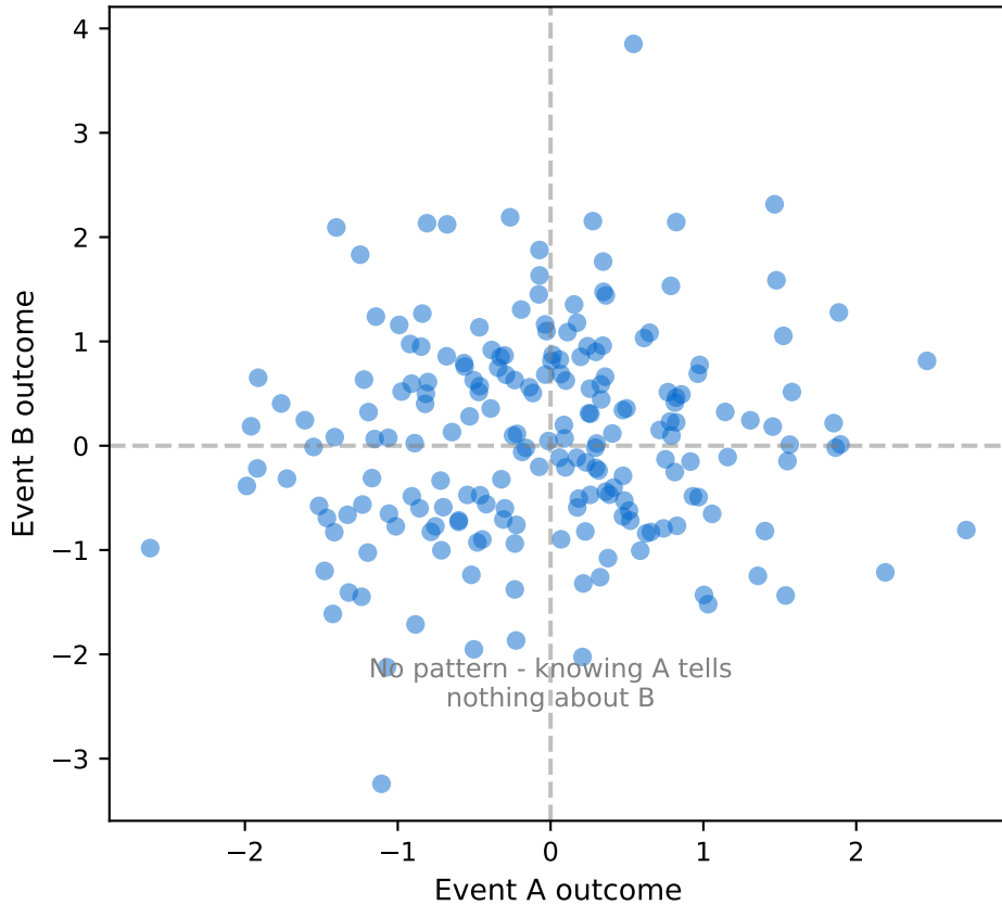
Independent Events P(A \text{ and } B) = P(A) * P(B)
