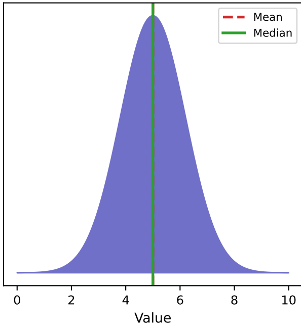
Symmetric (Zero Skew)
