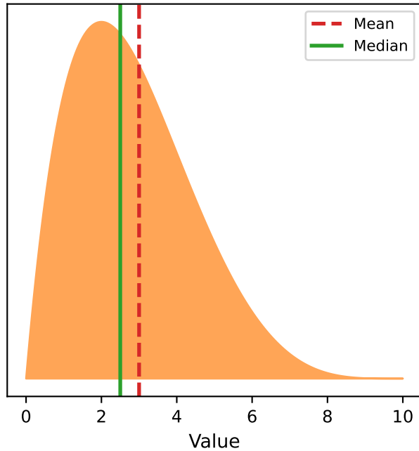
Right-Skewed (Positive Skew)
