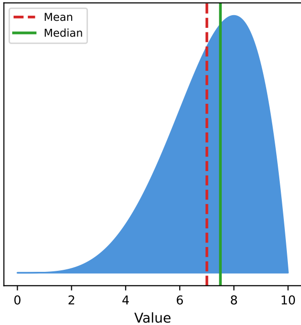
Left-Skewed (Negative Skew)
